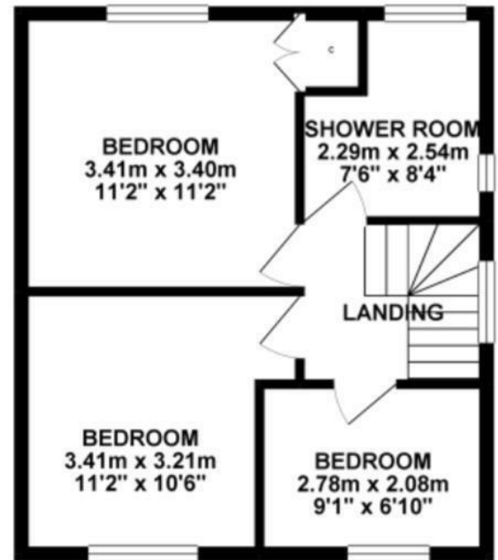
1ST FLOOR 37.64 sq. m. ( 405.12 sq. ft. )
